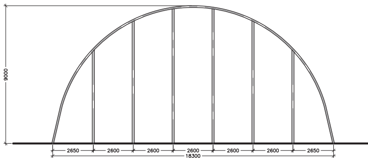
GABLE ELEVATION NTS
