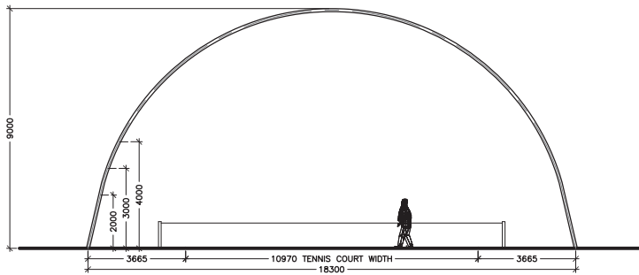
TYPICAL SECTION NTS
