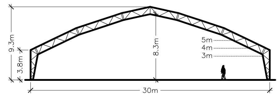
S-SPAN - 30M S-SPAN STRUCTURES ARE MODULAR ON 6M BAYS
