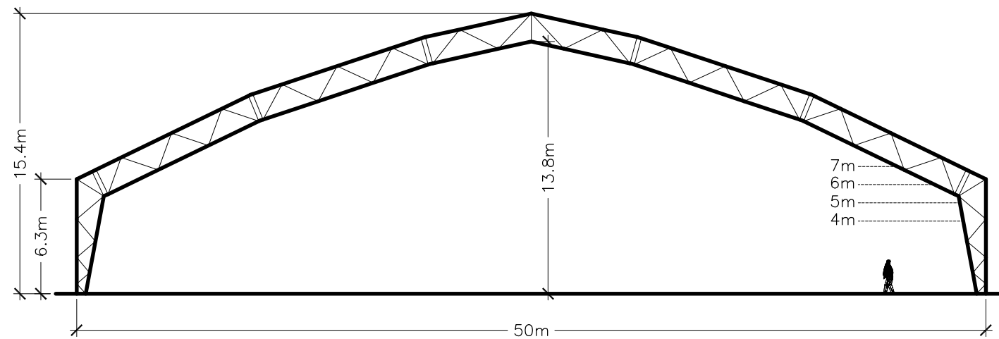
S-SPAN - 50M S-SPAN STRUCTURES ARE MODULAR ON 6M BAYS
