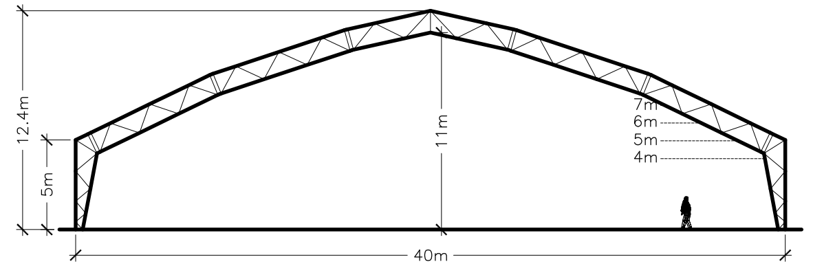
S-SPAN - 40M S-SPAN STRUCTURES ARE MODULAR ON 6M BAYS
