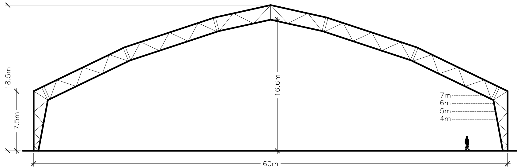
S-SPAN - 60M S-SPAN STRUCTURES ARE MODULAR ON 6M BAYS
